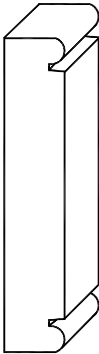
CH-325 9/16" X 3-1/4"
